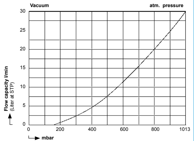
FLOW CAPACITY
